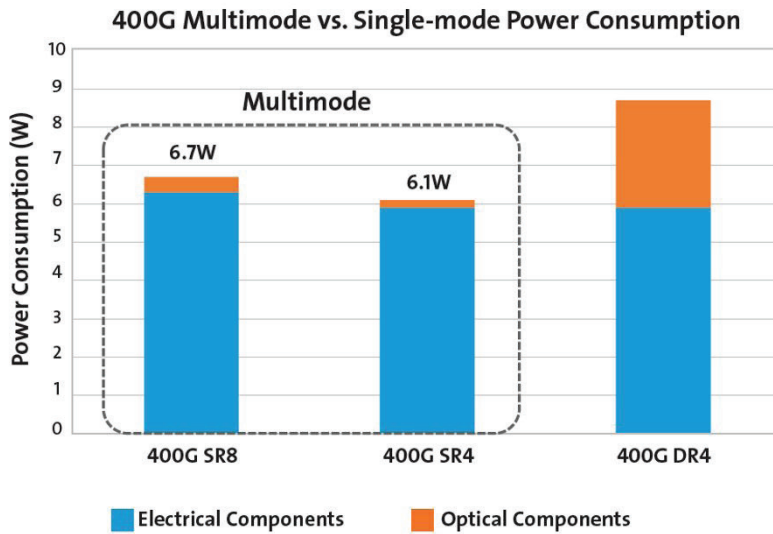
Figure 4. Multimode vs. Single-mode 400G Transceiver Power Consumption Comparison
