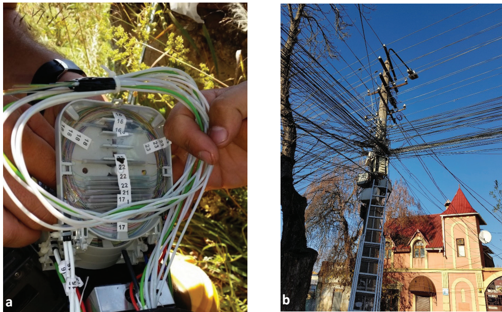
Figure 4. Examples of Installation Error Leading to Undesirably Tight Fiber Bending a) Small Bend Radius in Splice Closures b) Aerial Cable Deployment
