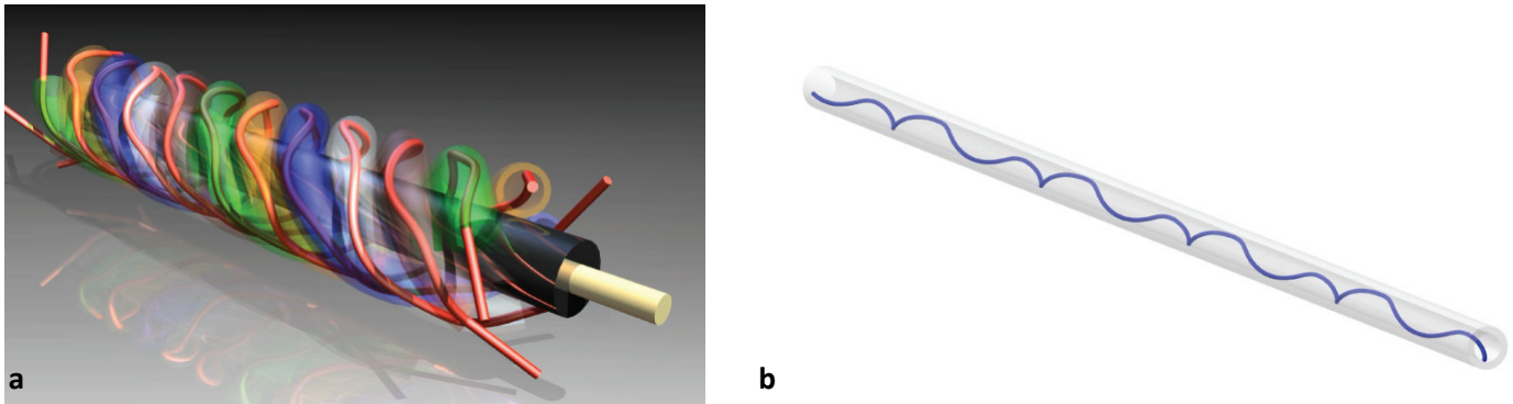
Figure 3. Simulated Picture of Fiber Curvature Under Environmental Conditions (Stress, Low Temperature) (a) Along the Cable Length; (b) Inside the Loose Tube
