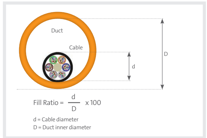
Figure 19A. Conduit Fill Ratio Calculation for Blowing Cable
