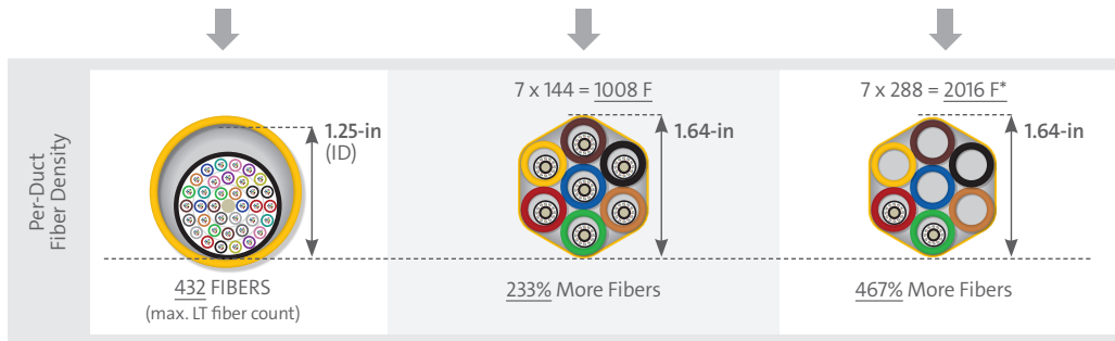
Figure 4. Comparison of Standard Loose Tube/Standard Duct, MiniXtend/MicroDuct, and MiniXtend HD/Microduct
