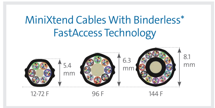
Figure 8. MiniXtend Cables With Binderless FastAccess Technology by Fiber Count
