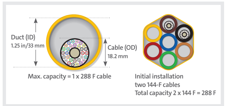
Figure 7. Standard 288-Fiber Loose Tube Cable Placed in a Standard Duct Compared to Two 144-Fiber Cables Placed in a Microduct System
