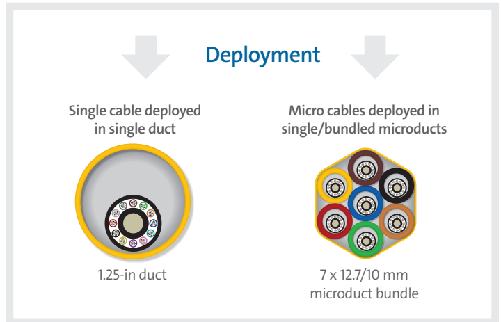
Figure 2. Comparison of Single Cable Deployed in a Single Duct to Micro Cables Installed in a 7-Way Duct
