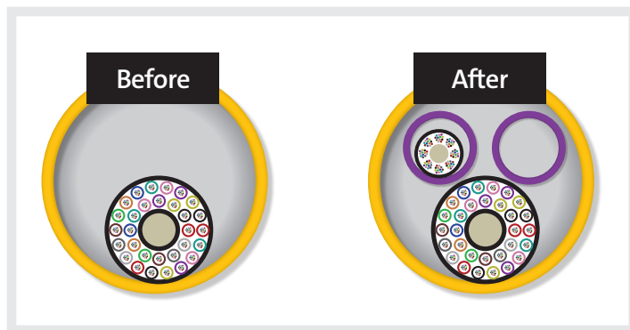
Figure 27. Before and After of an Existing Duct With a Cable Installed and Two New Microducts Installed
