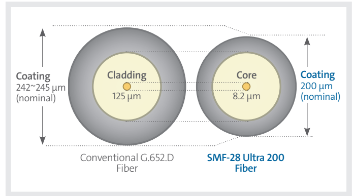
Figure 14. Comparison of Conventional G.652.D Fiber and Corning SMF-28 Ultra 200 Fiber
