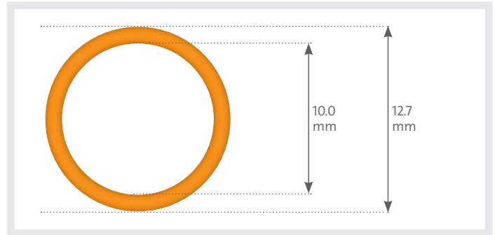
Figure 19. Microduct Naming Convention
