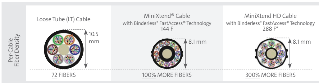
Figure 3. Comparison of Standard Loose Tube Cable, MiniXtend Cable, and MiniXtend HD Cable
