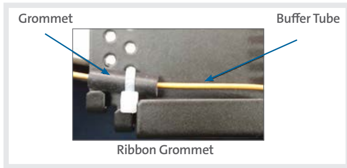
Figure 20. Ribbon Strain-Relief Kit
