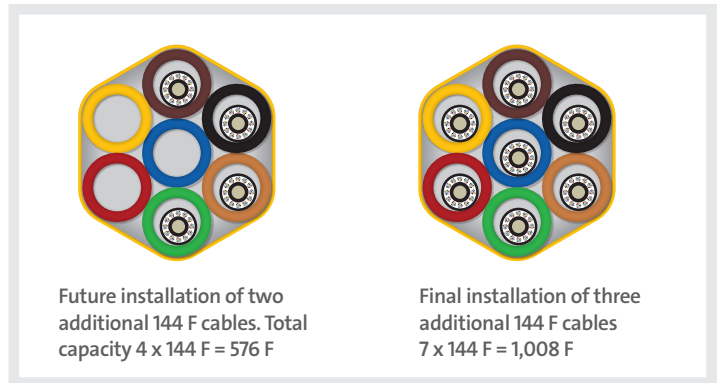
Figure 8. Upgrade Path Utilizing a 144-Fiber Cable in Microducts
