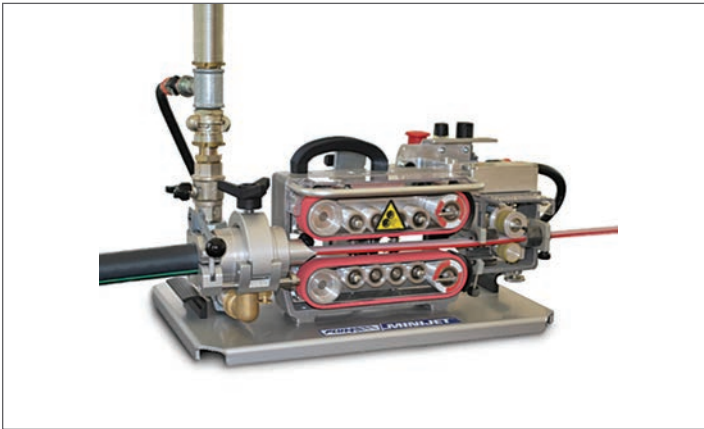
Figure 22. Micro Cable Blowing Machine
