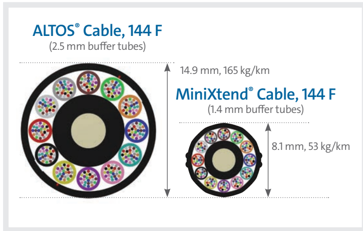
Figure 1. Comparison of Standard 144-Fiber Loose Tube Cable to a 144-Fiber MiniXtend Cable
