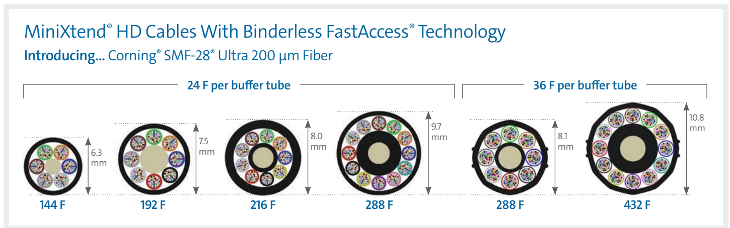
Figure 13. MiniXtend HD Cable by Fiber Count
